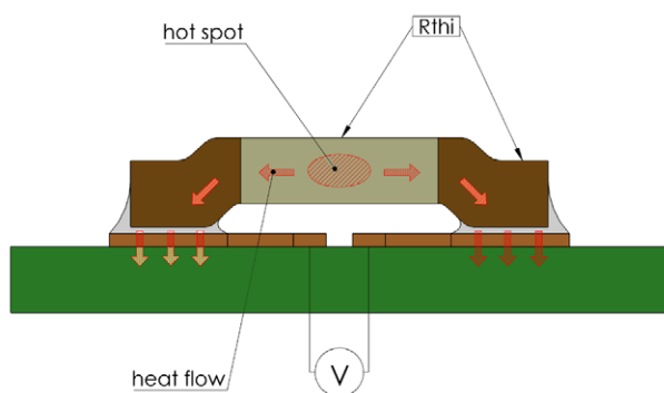
Figure 4: The heat development in the component: Temperature difference between the hot spot and contact point
