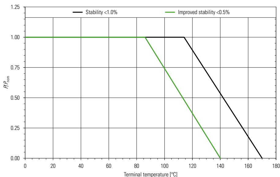
Figure 5: Power derating curve for the component BVT-M-R001
