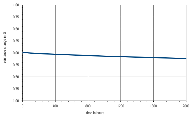
Figure 6: Typical wave form for the long-term stability of the component BVS-M-R0005-1.0
