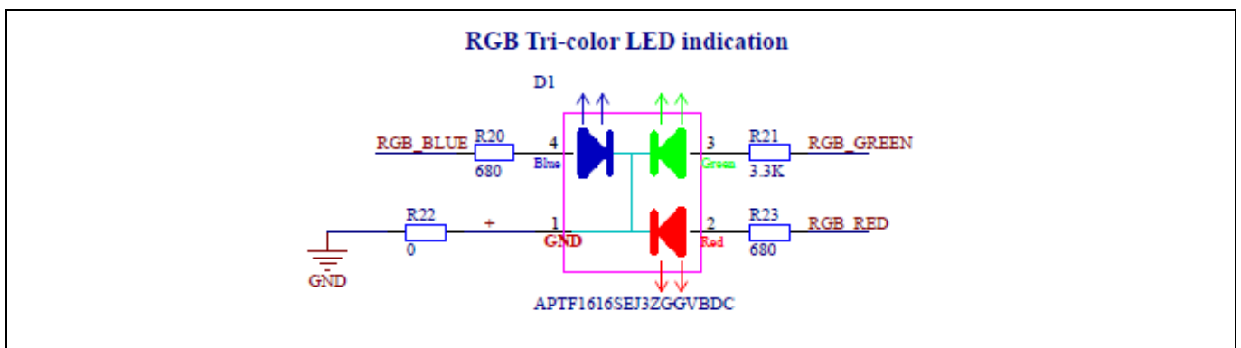
Figure 12 LEDs schematic
